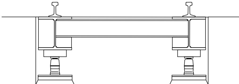
7260 Cross Section
